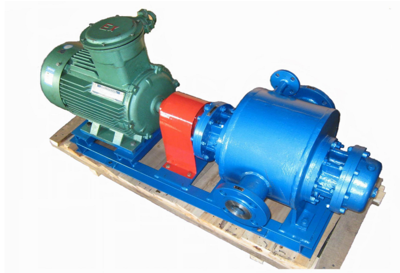
Twin-screw pump with thermal insulation sleeve
